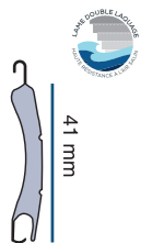
8 mm RS 41 SW Lame Alu
